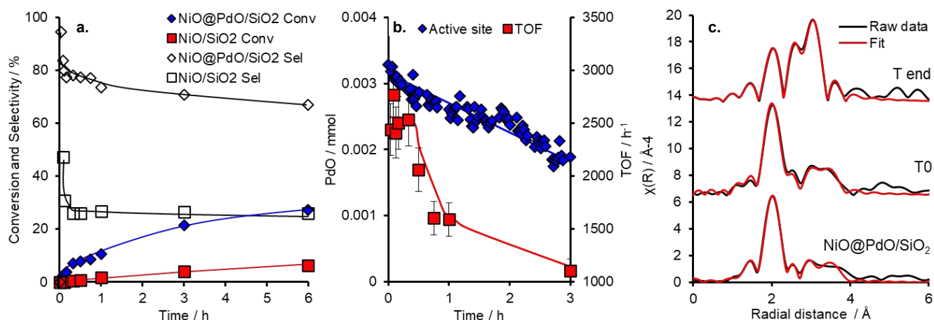
Figure 3. a. Selox reaction and selectivity profiles for NiO@PdO/SiO 2 and NiO/SiO 2 , b. evolution of catalytic PdO content and instantaneous TOFs derived from LCF of operando Pd K edge XAS during cinnamyl alcohol selox, and c. FT EXAFS and fit of ex-situ and operando NiO@PdO/SiO 2 at T 0 and 6 hours.
