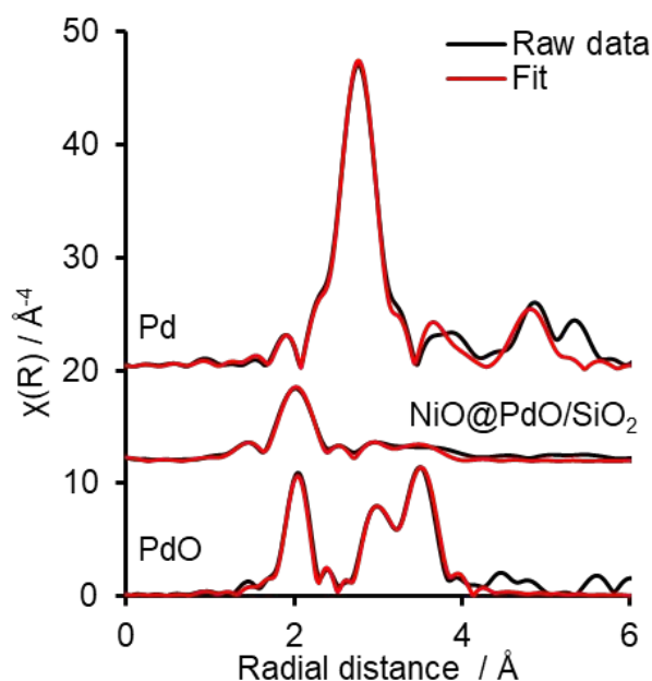
Figure 2. EXAFS Fourier transforms and fits for PdO and Pd references and NiO@PdO/SiO 2 .
