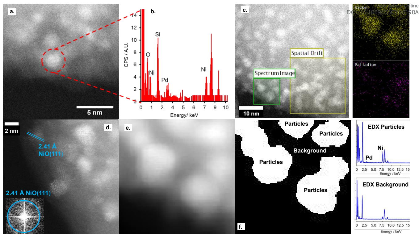
Figure 1. a. High-angle annular dark field (HAADF)-STEM of NiO@PdO/SiO 2 , b. selected area energy dispersive X-Ray (EDX) spectrum of highlighted nanoparticles, c. EDX mapping of NiO@PdO/SiO 2 , d. atomic resolution imaging of NiO@PdO/SiO 2 with Fourier transform of the STEM image (inset), and e. and f. HAADF-STEM imaging and applied particle and background mask for EDX spectra subtractions with corresponding EDX spectra.
