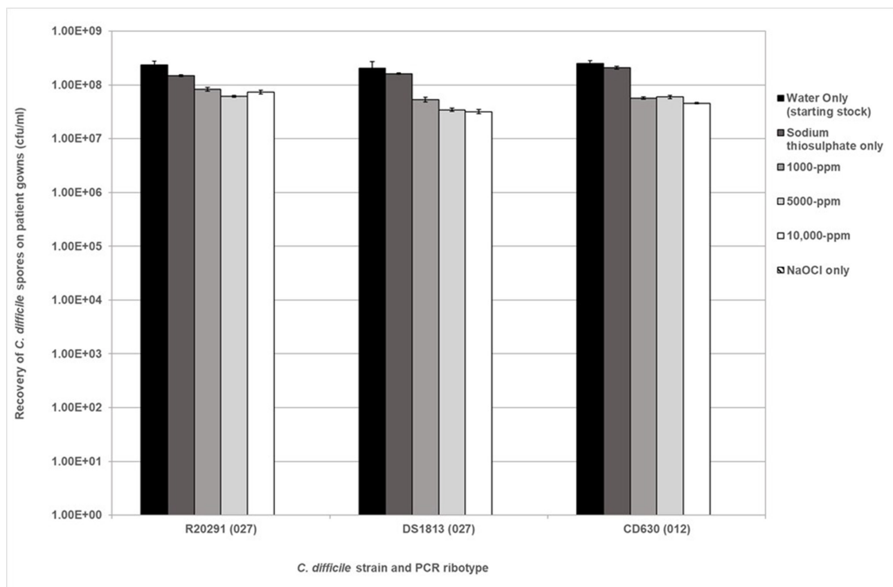
Fig. 5. Recovery of purified C. difficile R20291, DS1813 and CD630 spores from spiked patient gowns following exposure of 10^9 c.f.u. ml^{-1} to NaOCl at 1000, 5000 and 10 000 p.p.m. for 10 min. Spores not exposed to NaOCl (water only) were used as a positive control and the use of NaOCl only was used as a negative control, where no spores were recovered. Plots represent mean \pm SEM ( n=3 ).
