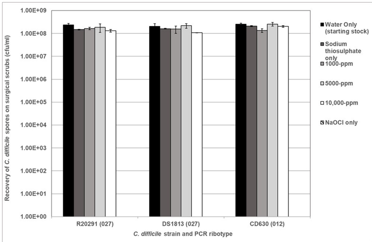
Fig. 4. Recovery of purified C. difficile R20291, DS1813 and CD630 spores from spiked surgical scrubs following exposure of 10^8 c.f.u. ml -1 to NaOCl at 1000, 5000 and 10 000 p.p.m. for 10 min. Spores not exposed to NaOCl (water only) were used as a positive control and the use of NaOCl only was used as a negative control, where no spores were recovered. Plots represent mean \pm SEM ( n=3 ).
