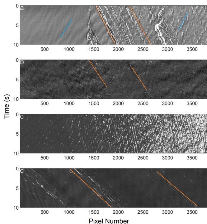
Fig. 18. Pixel timestacks for greyscale intensity, timestacks are orientated such that the current direction is from left to right. a) Mumbles Head; b) Flood from Ramsey Sound 12th; c) Ebb from Ramsey Sound on the 12th; d) Flood from Ramsey Sound on the 14th. Where the current is evident, orange lines illustrate the travel of some current signatures; in panel a, the blue lines indicate wave signatures in the timestack.
