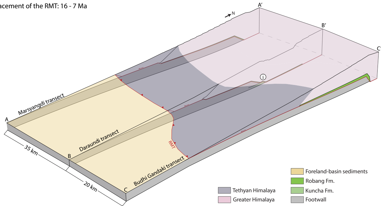
Predicted thermochronology
