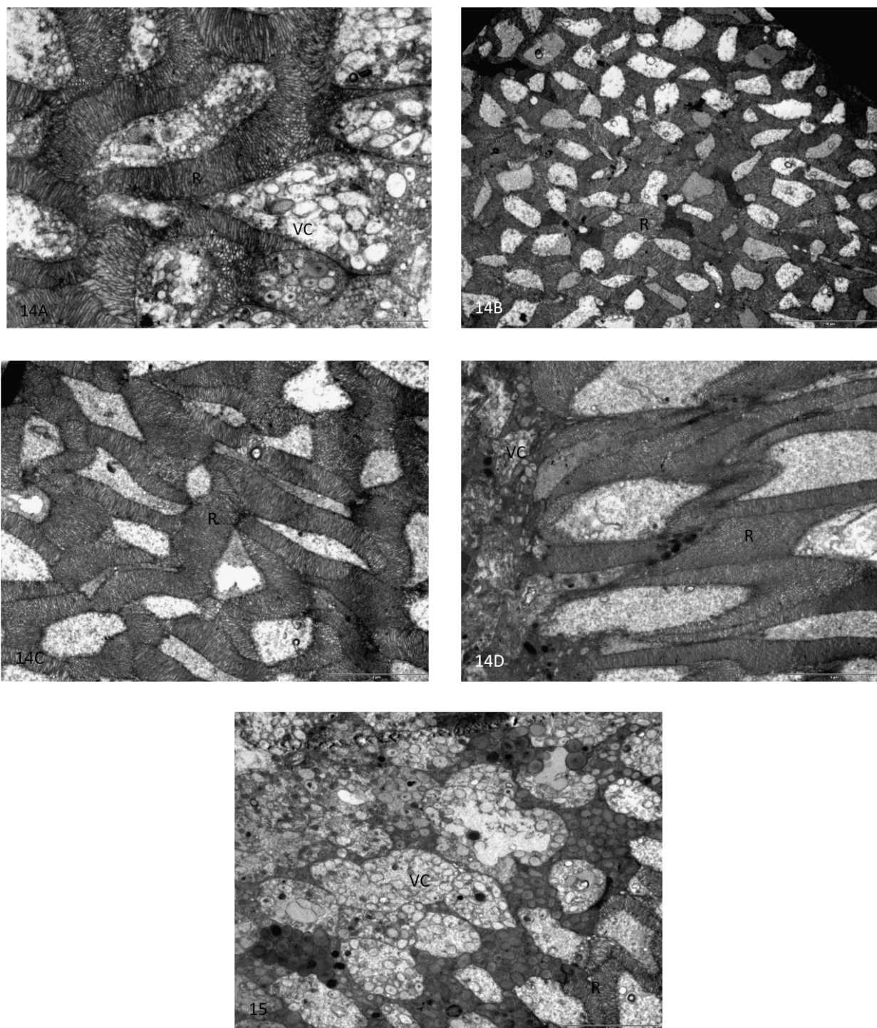
Fig. 14 TEM image of the dark reared retina. A transect through the retina started in the middle of the eye working through the outer segment. (A) Start of outer segment. Scale bar = 2 \mu m. (B) Small compacted rhabdomeres at beginning of outer segment. Scale bar = 10 \mu m. (C) Middle of the outer segment as rhabdomeres start to elongate. Scale bar = 5 \mu m. (D) End of outer segment and beginning of sub-rhabdomeric layer. Scale bar = 5 \mu m. (R) rhabdomeres, (VC) vesicle cells.
