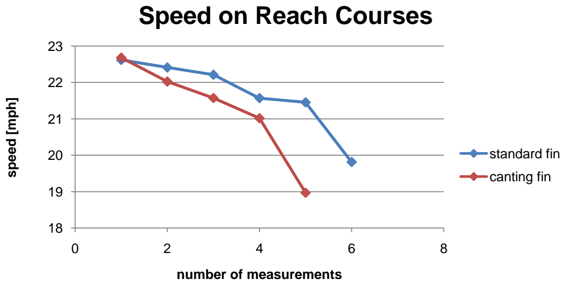
Figure 13. Comparison of speeds on reach courses
