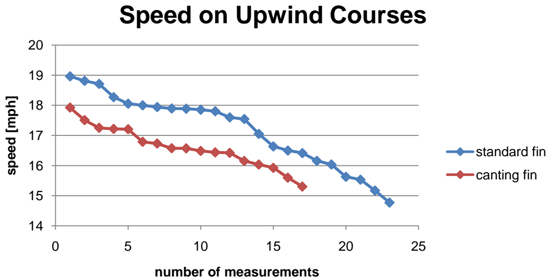
Figure 12. Comparison of speeds on upwind courses
