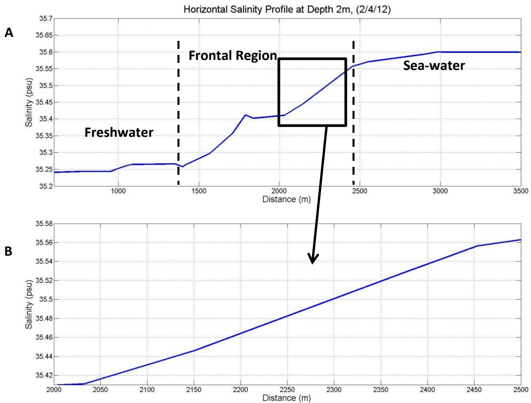
Figure 5: 5A and B show a horizontal salinity profile at a depth of 2m, from Plymouth breakwater to L4, on 02/04/12. '5A' is the complete profile and outlines the 3 bodies of water. '5B' is an enlarged image of the outlined section, the last sharp salinity gradient, within the frontal region.
