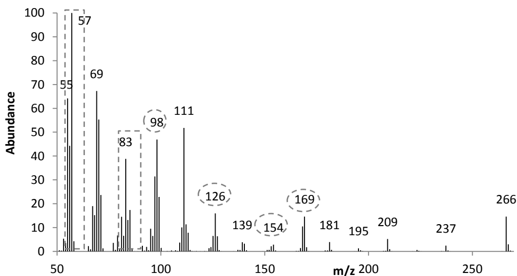
Figure 31: Mass spectrum of the peak at 15:41 min; isomer of 5-ethyl-7-butyltridecene
