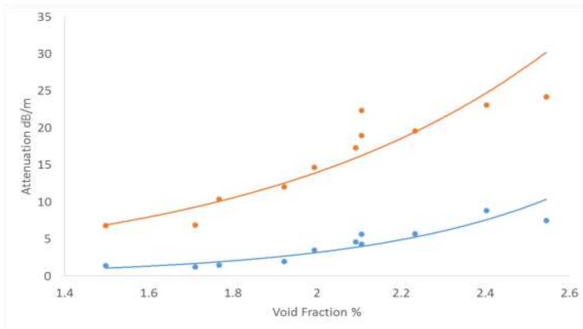
Figure 5.18: Attenuation at 500 kHz (blue) and 195 kHz (orange) against void fraction within the bubble cloud.
