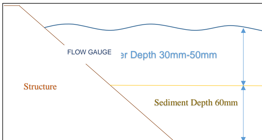
Figure 5: Cross section at end of structure showing sediment layer
