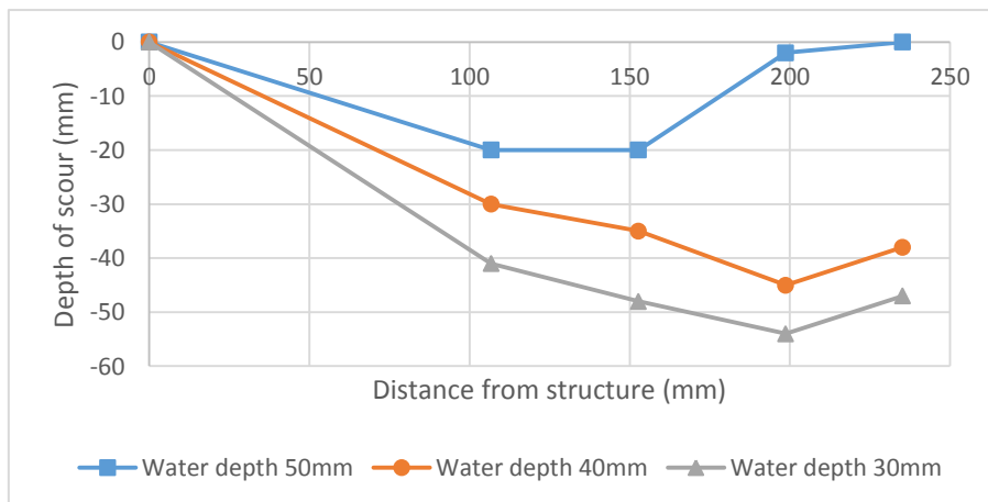
Figure 16: Graphical representation of scour depths from the end of the Mount Batten model for varying water depths.
