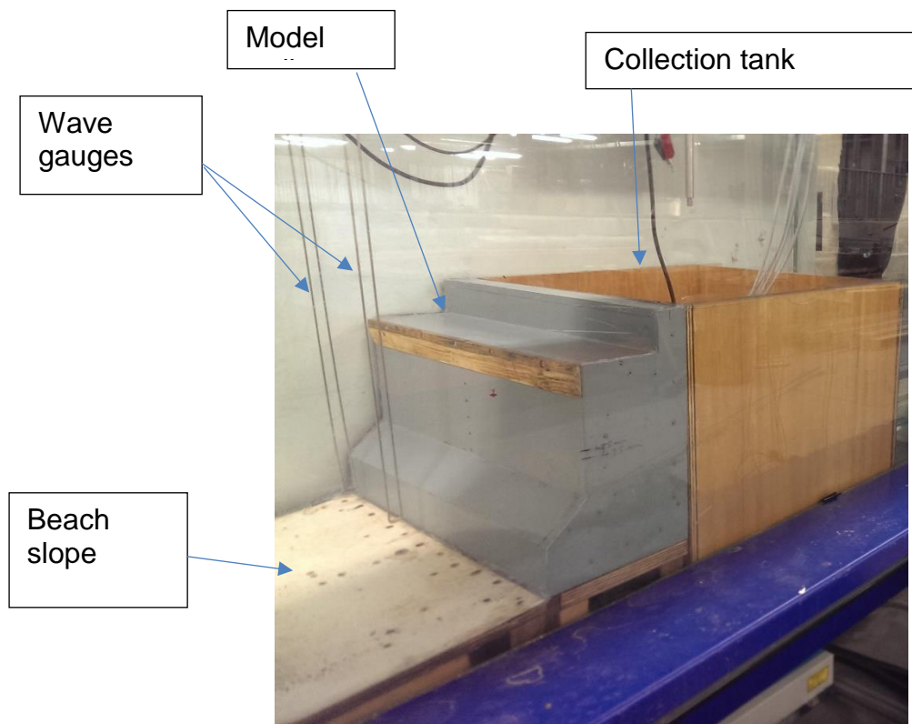
Figure 1: Model setup
