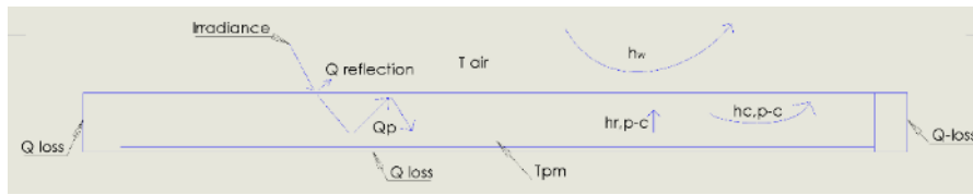
Figure 2: Assumed losses (Chekerovska & Filkoski, 2015)
