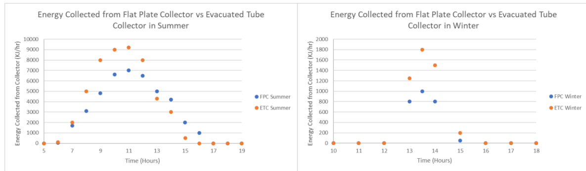
Figure 12: Energy Collected from Flat Plate Collectors and Evacuated Tube Collectors in Summer and Winter Simulated in TRNSYS
