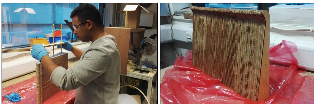
Figure 4: Gluing the offcuts and aligning them with the use of dowels
