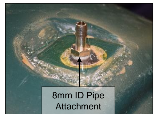
Figure 31: 8mm pipe attachment
