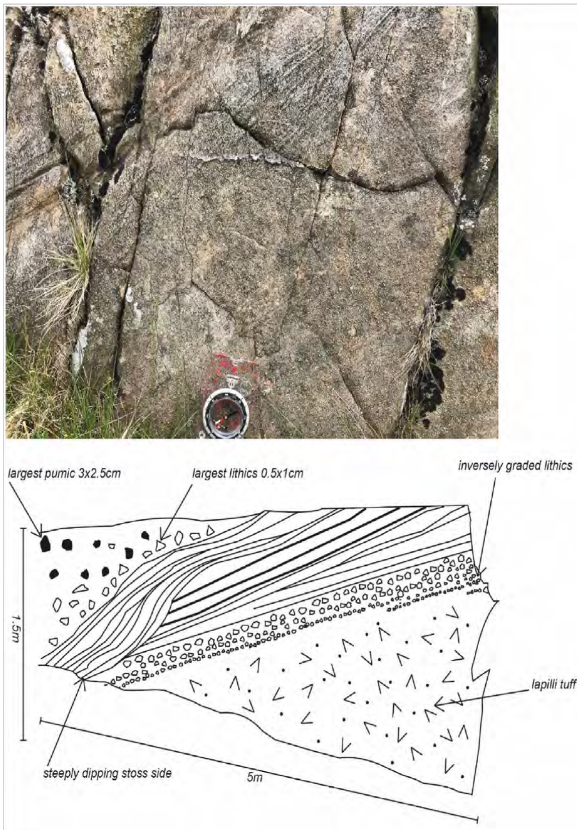
Figure 3.6 Buck Pike Tuff and Clastic Fmt. GR: 26214, 94863. Geological sketch accompanying a field photo of a chute and pool structure with a palaeocurrent of 185° observed in the lapilli tuff member.
