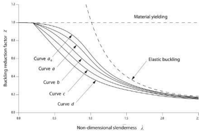
Figure 4: Buckling Reduction Factor vs. Non-Dimensional Slenderness (Stibor, 2014)
