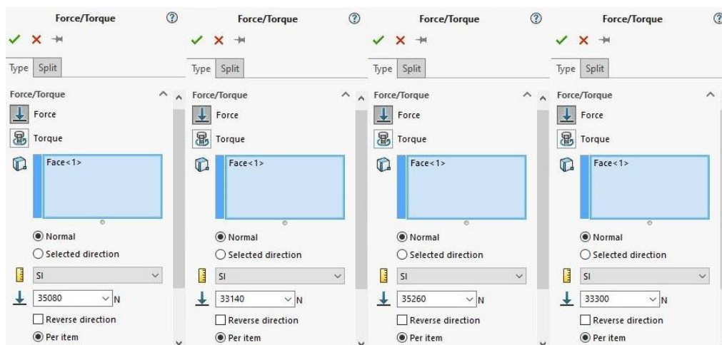
Figure 5: Axial Compressive Force Values
