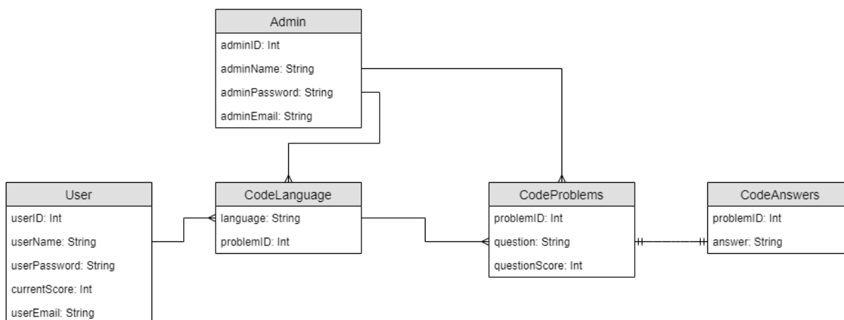
Initial ERD - Sprint 3
