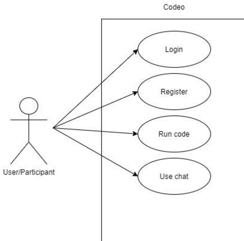
Figure 8: UML Diagram of the Research Application
