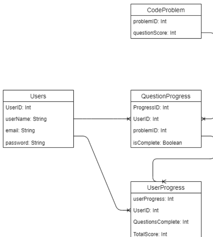
Figure 11: Finalised database entity relationship diagram for research tool.
