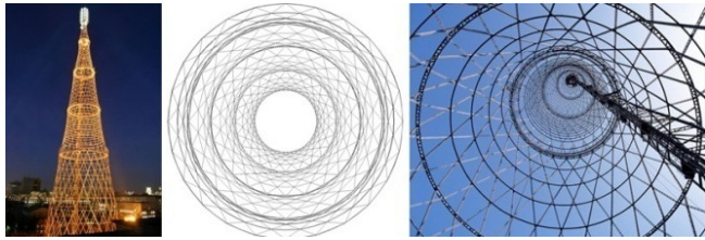
Figure 1: The hyperboloid structure of Shukhov Tower.
