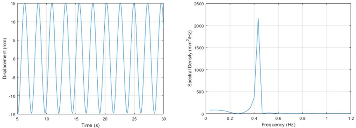
Figure 6: Displacement & Spectral Density – 0.43Hz, 30mm Surge
