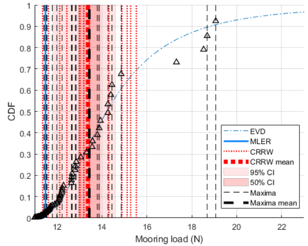
Figure 10: EVD of the front mooring load, the shading shows the 50 and 95% confidence intervals. The triangles show the empirical EVD of the peaks from the irregular waves which the EVD is predicted from. 20 CRRW responses are shown. The dashed lines labelled maxima show the largest response from each of the 18 irregular wave seeds.
