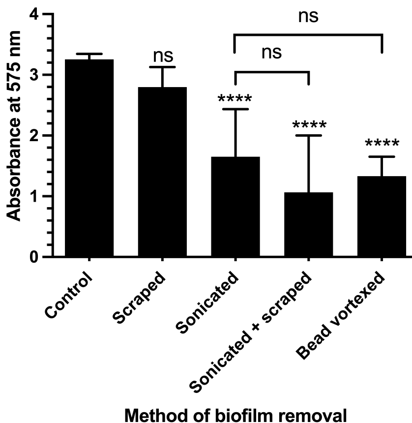
Figure 4.5: Crystal violet solubilisation assay of uncoated uPVC discs following 24 h incubation with Pseudomonas aeruginosa NCIMB 10817 and attempts by different methods to remove biofilm. The control group represents discs where no attempt was made to remove biofilm. Data presented as mean \pm standard deviation. **** p < 0.0001 , ns = not significant; one-way ANOVA compared to control with Tukey's multiple comparisons test. Data presented are the average of n=2 biological replicates.
