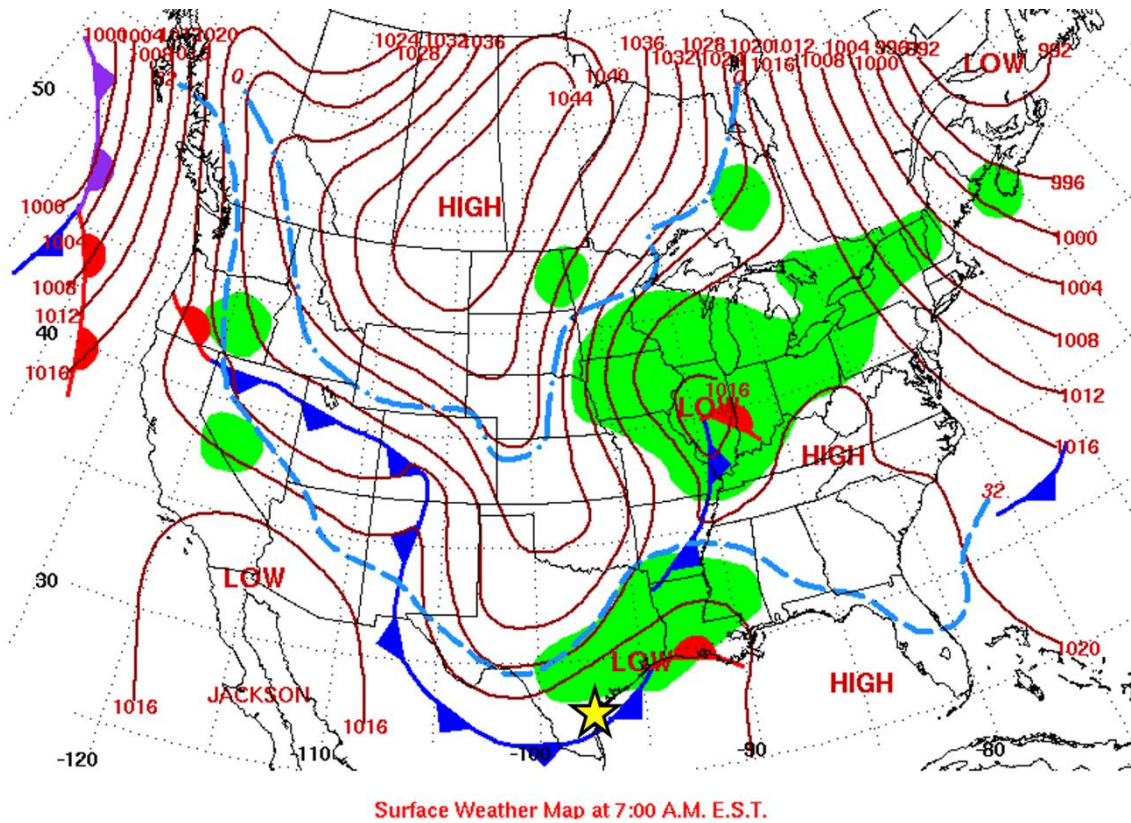
Figure 9: Daily U.S surface weather map for 07/01/2010 at 7:00 a.m. E.S.T showing the formation and progression of cold fronts (solid blue line with triangles) and warm fronts (solid red line with semi-circles) around regions of high (H) and low (L) pressure across the United States with resulting precipitation (green shaded regions) (NOAA Weather Prediction Center, 2022). The location of Corpus Christi Bay Texas is indicated by the yellow star marker.
