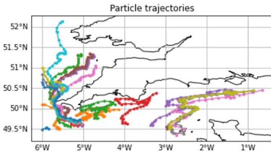
Figure 9: Trajectories of particles run from the random starting line 5^{\circ}5:49^{\circ}2 and -3^{\circ}:49^{\circ}75 between the 1st of October and 20th December of 2018. Note that each color line represents the trajectory of each particle at the starting position showed in Figure 10 and finishing as seen in Figure 11. Simulation plotted on Ocean Parcels.
