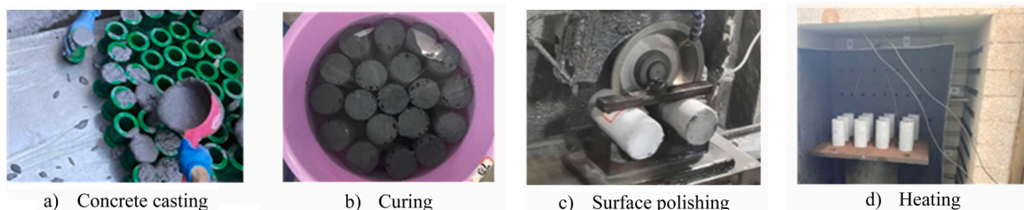
Fig. 2. Preparation of GPM and GPC specimens.
