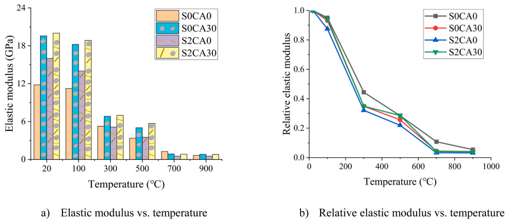
Fig. 16. Elastic moduli of GPM and GPC specimens after exposed to elevated temperatures.
