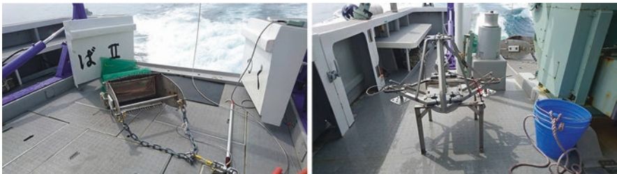
Fig. 22.5 Example of dredge, and grab sampling
