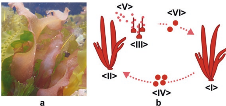
Fig. 12.11 The life cycle of Palmaria palmata . (a) Palmaria palmata . (b) Life cycle. <I>: sporophyte, <II>: male gametophyte, <III>: female gametophytes, <IV>: tetraspores, <V>: spermata, <VI>: carpospores
