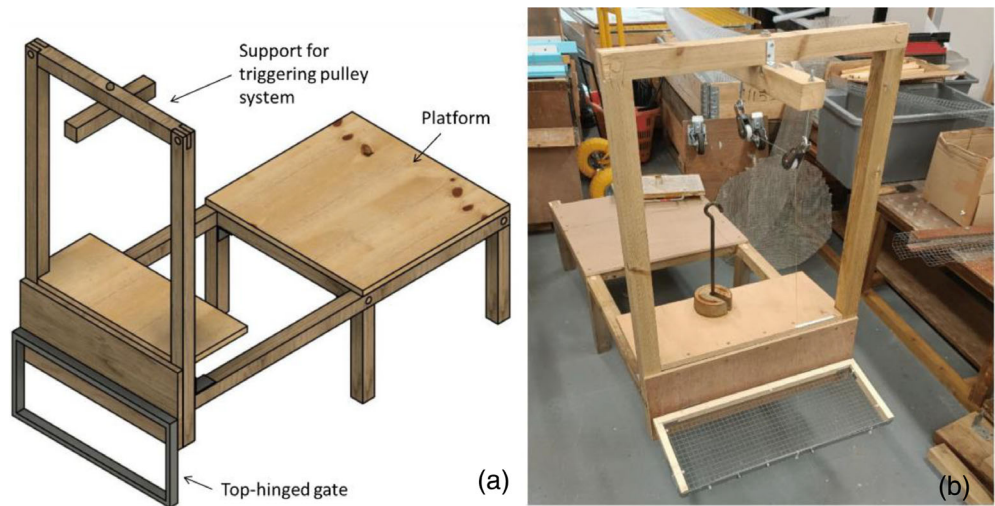
FIGURE 3 Setup B debris release mechanism (a) conceptual drawing (b) laboratory model.
