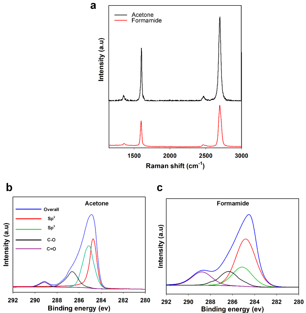
Figure 5- 2 Raman spectra (a) and XPS data (b and c) of graphene processed with acetone and formamide.
