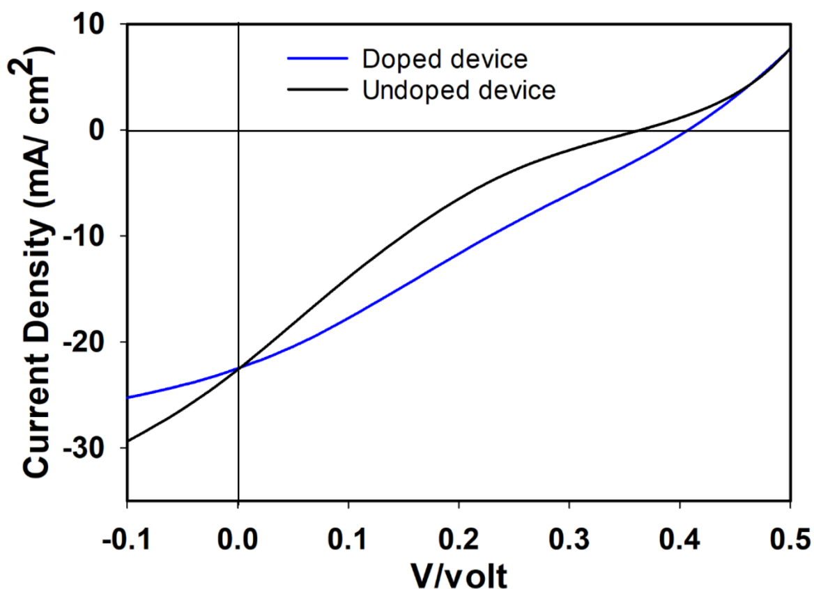
Figure 4- 9 J-V features of doped and undoped solar cells.
