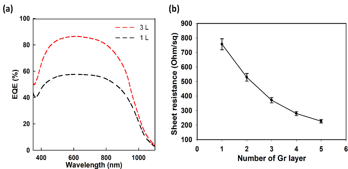
Figure 4- 13 (a) Curves showing EQE of solar cells constructed using a single layer and three layers. (b) Established sheet resistivity of multi-graphene layers.
