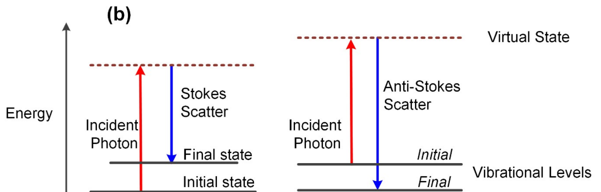
Figure 3- 3 (a) An image of Raman Spectroscopy. (b) A schematic of Stokes and anti-Stokes scattering processes.
